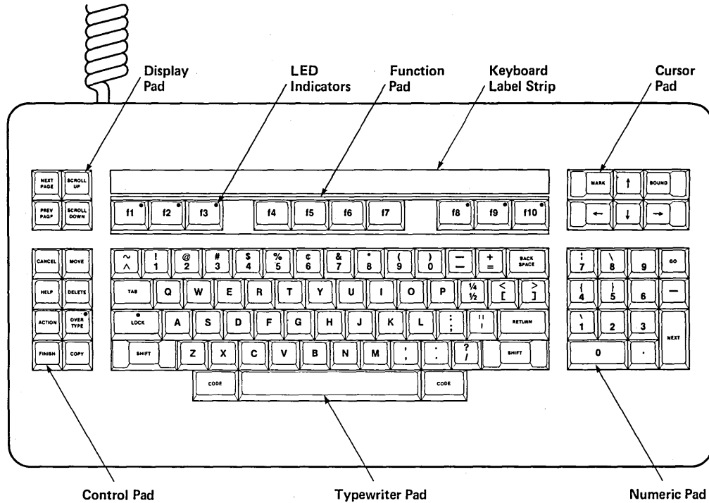
Figure 3-2. Keyboard.
